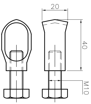
Clamp (copper)
