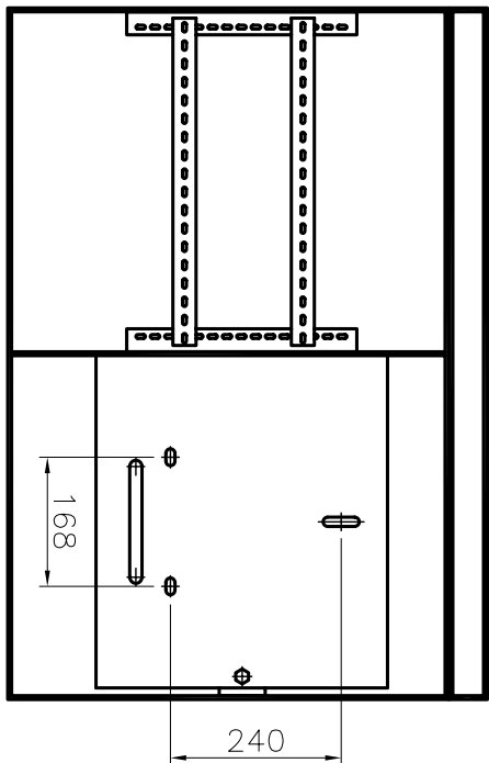
Front View (Open Door)
